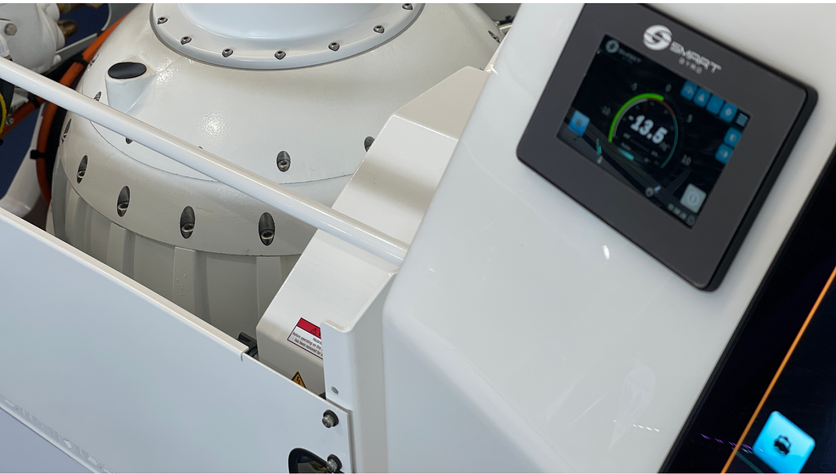
The Smartgyro SG series gyroscopic stabilizer
